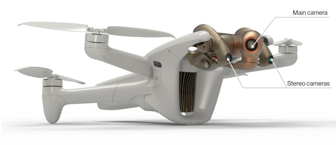
ANAFI Ai's dual gimbal for perception and imaging
